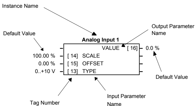
Figure Chapter 1-1 Function Block Parameter Information
